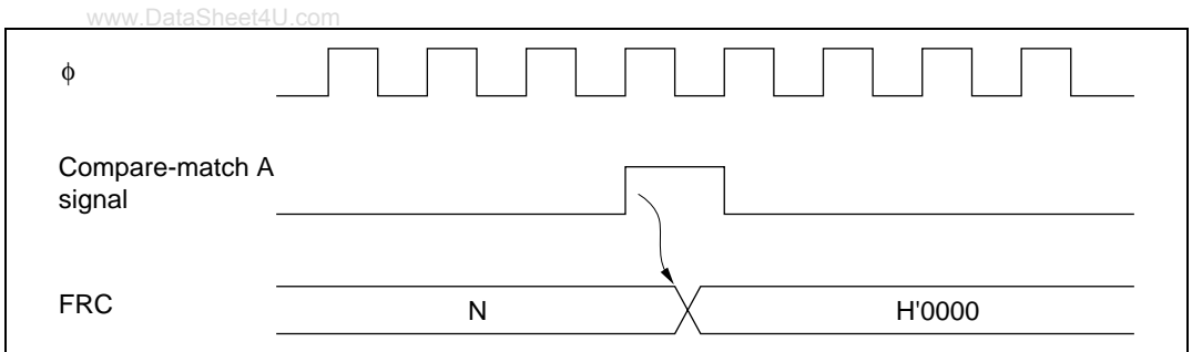
Figure 11.6 Clearing of FRC by Compare-Match A
