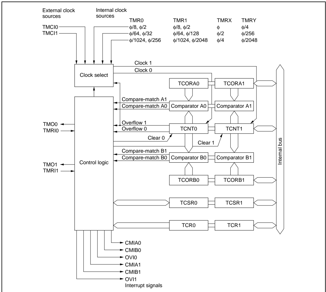
Figure 12.1 Block Diagram of 8-Bit Timer Module
