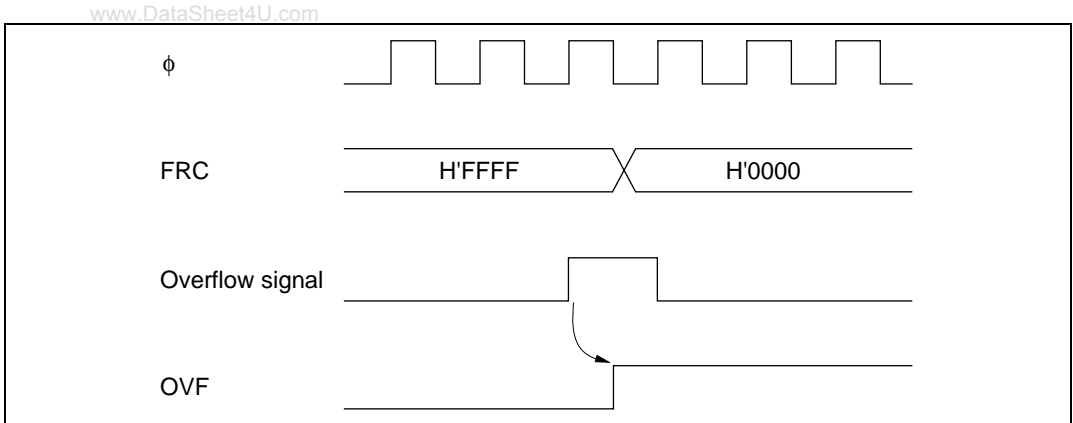
Figure 11.13 Setting of Overflow Flag (OVF)
